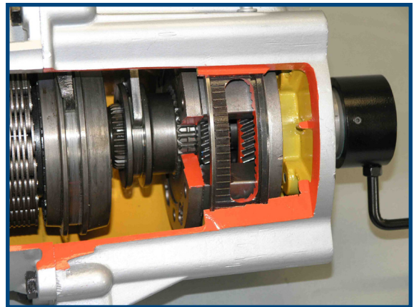
Transfer Case (High Range Position) Close-Up (model 1230)
